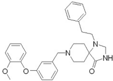
PC-6097201, CDCl 3
